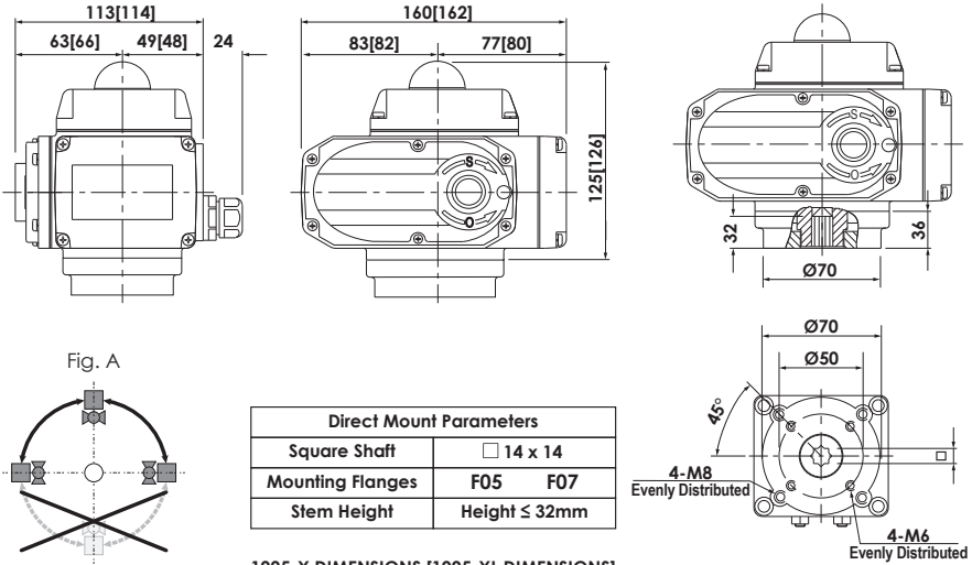
1005-X DIMENSIONS [1005-XL DIMENSIONS] 1005/S-X DIMENSIONS [1005/S-XL DIMENSIONS]
