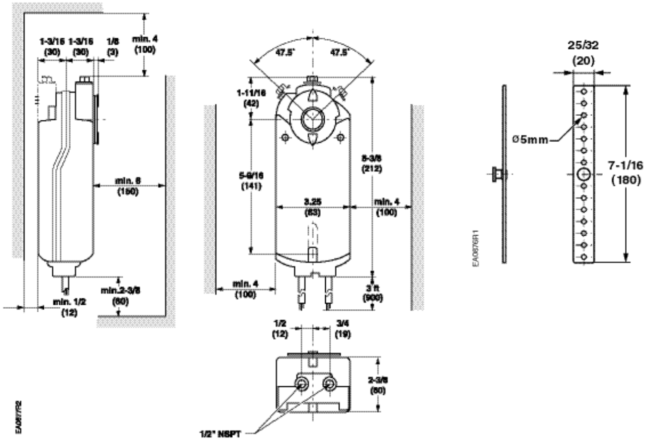
Figure 22. GMA Actuator and Mounting Bracket Dimensions.
