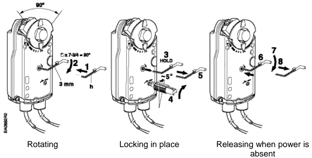
Figure 9. Manual Override.
